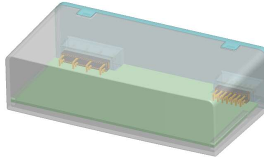
2. 3D View
